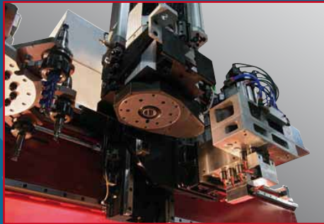
'Rotor' axis system to allow continuous 360° rotation of angular aggregates.
